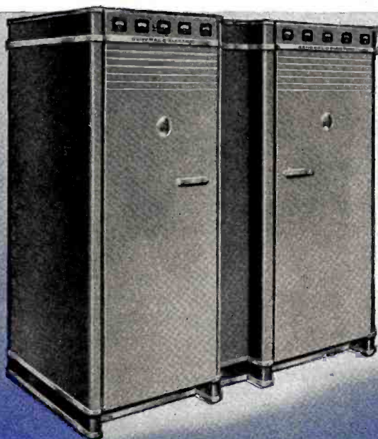
G-E 1 KW FM BROADCAST TRANSMITTER
